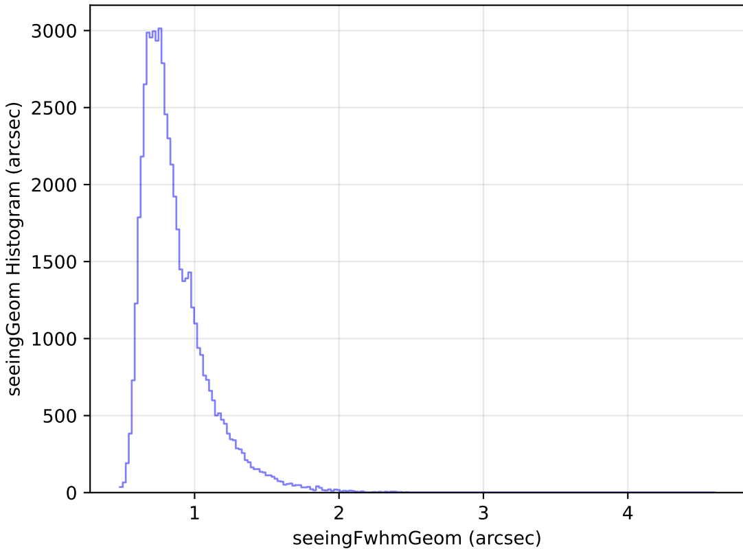
roll_pause_mjdp0_v3.4_10yrs Yr 1 i band: seeingGeom Histogram
