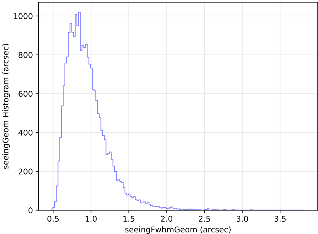
roll_pause_mjdp0_v3.4_10yrs Yr 1 g band: seeingGeom Histogram
