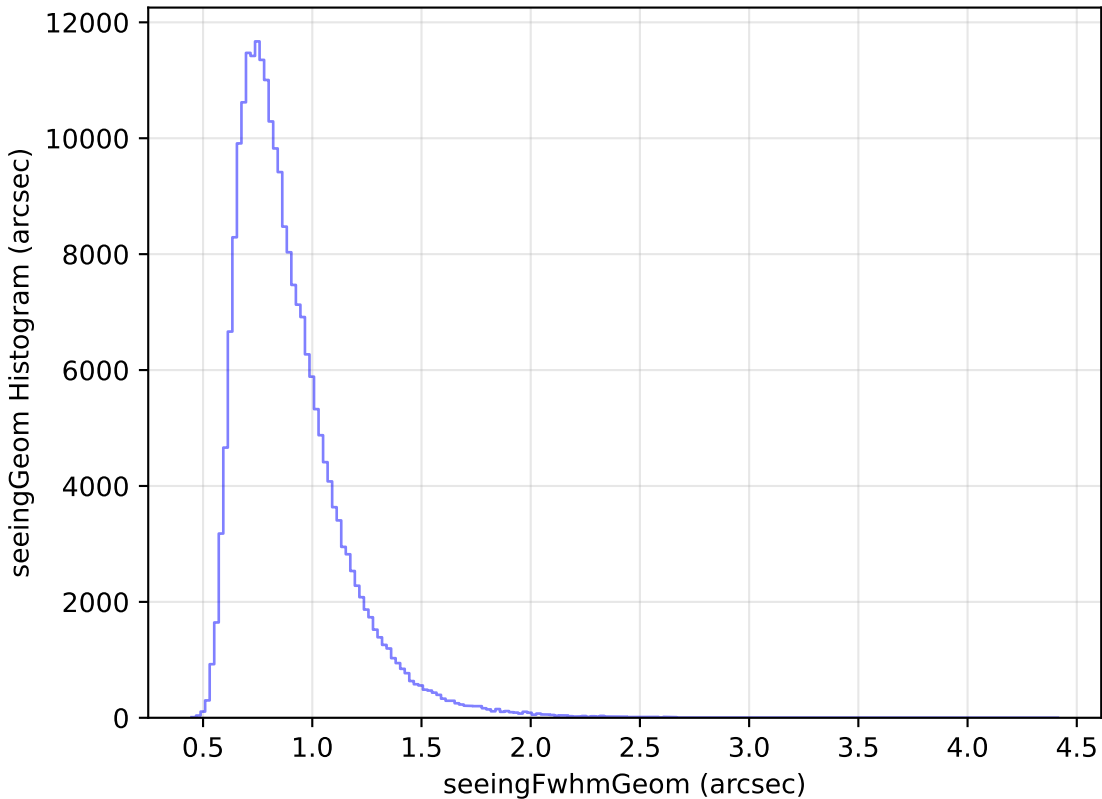
roll_pause_mjdp0_v3.4_10yrs Yr 1 all bands: seeingGeom Histogram
