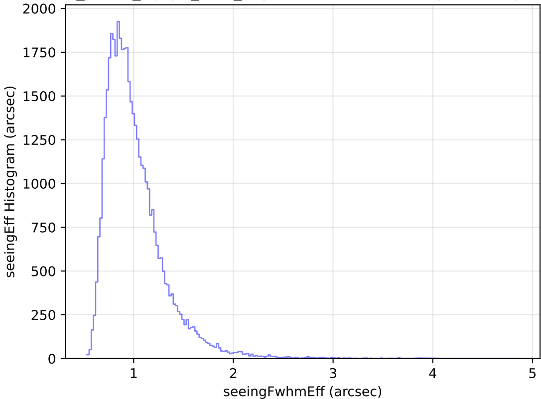
roll_pause_mjdp0_v3.4_10yrs Yr 1 z band: seeingEff Histogram
