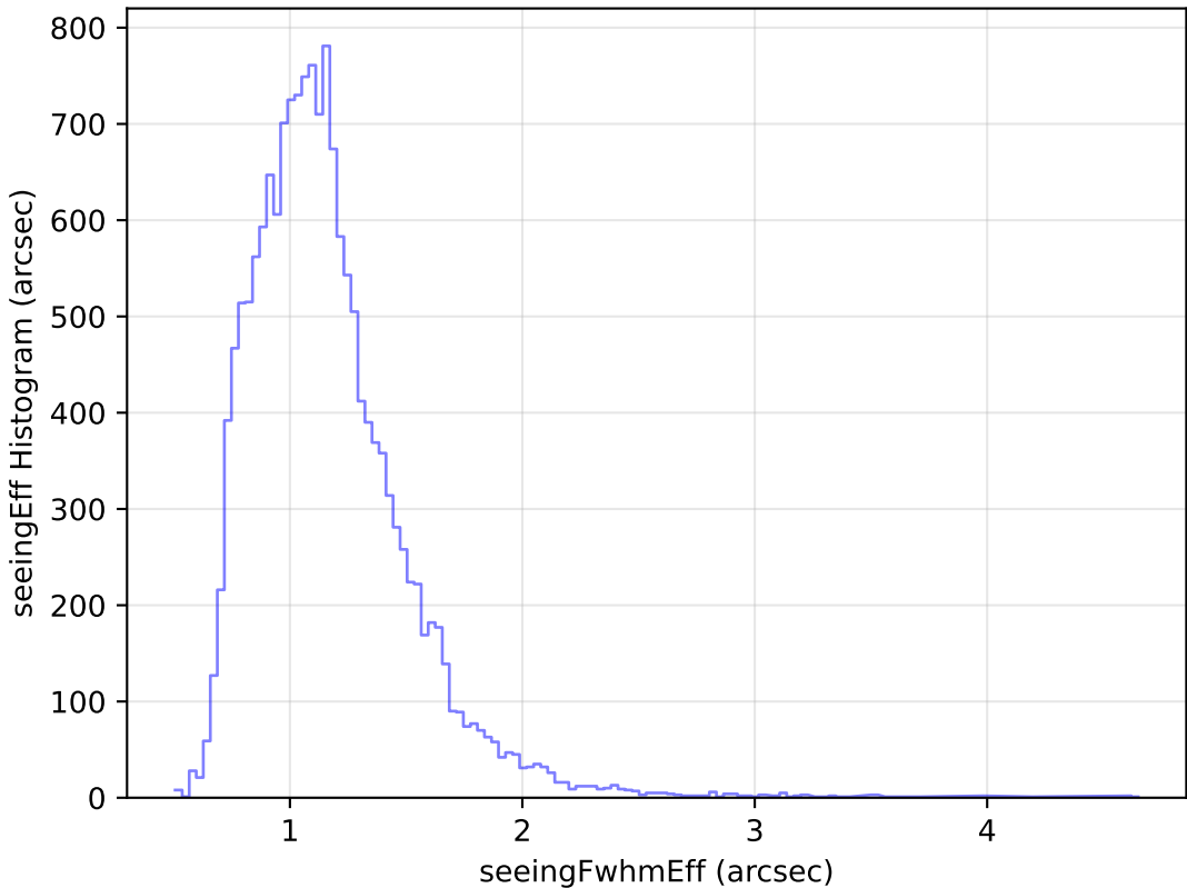
roll_pause_mjdp0_v3.4_10yrs Yr 1 u band: seeingEff Histogram
