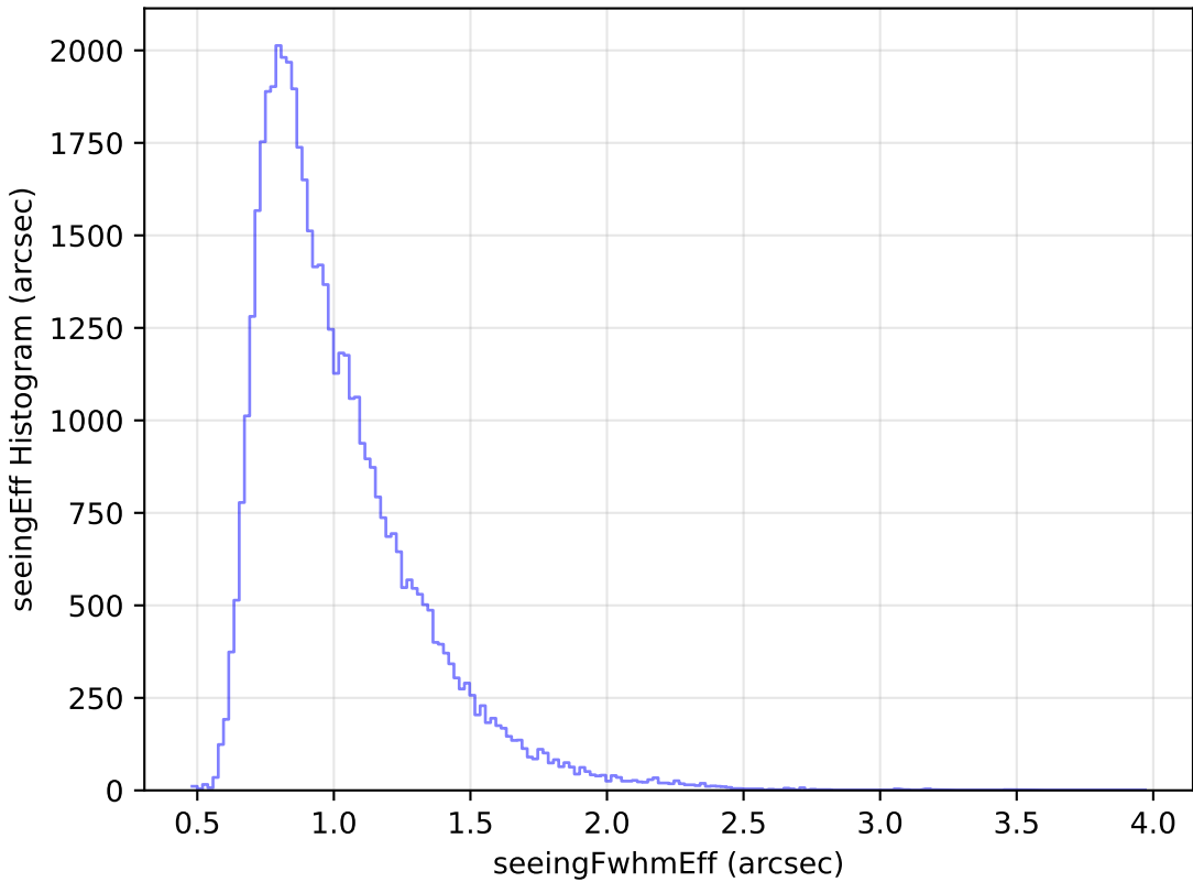
roll_pause_mjdp0_v3.4_10yrs Yr 1 r band: seeingEff Histogram
