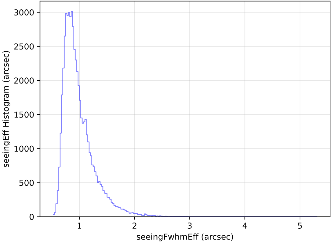
roll_pause_mjdp0_v3.4_10yrs Yr 1 i band: seeingEff Histogram
