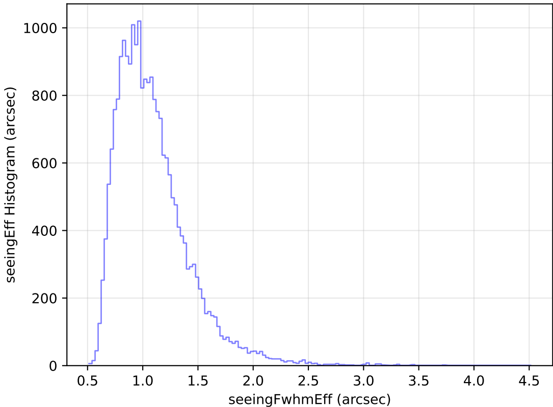
roll_pause_mjdp0_v3.4_10yrs Yr 1 g band: seeingEff Histogram
