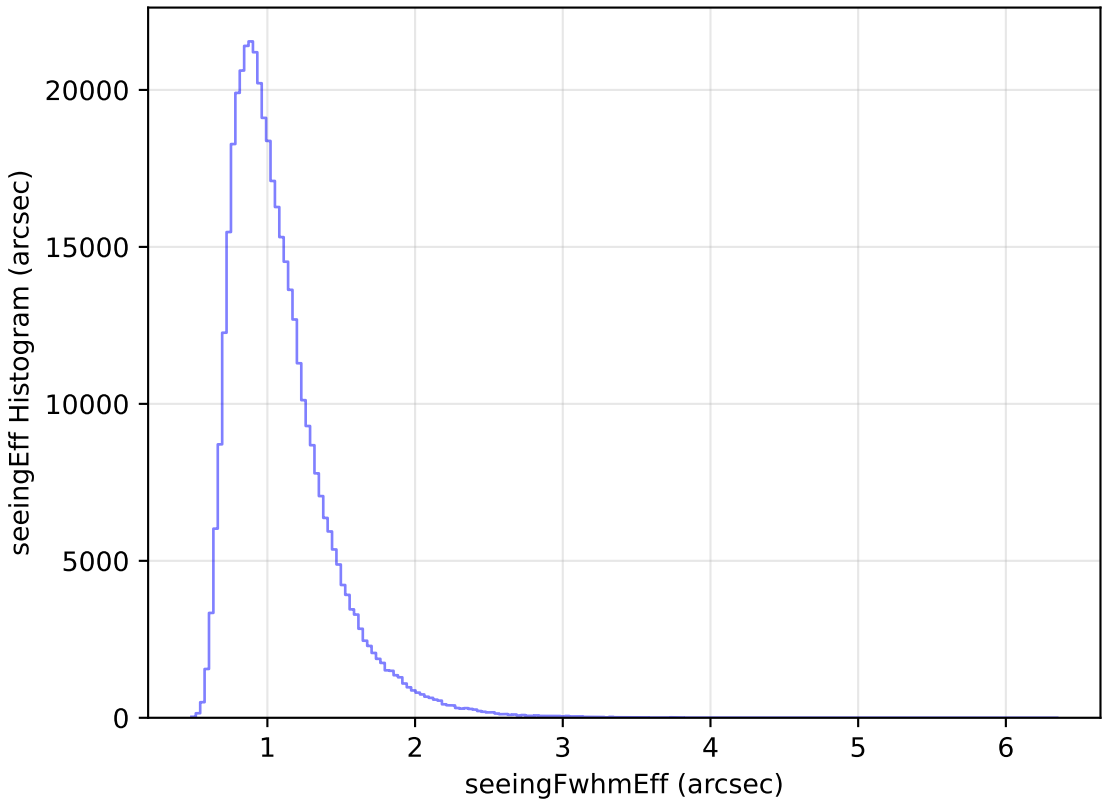
roll_pause_mjdp0_v3.4_10yrs WFD z band: seeingEff Histogram
