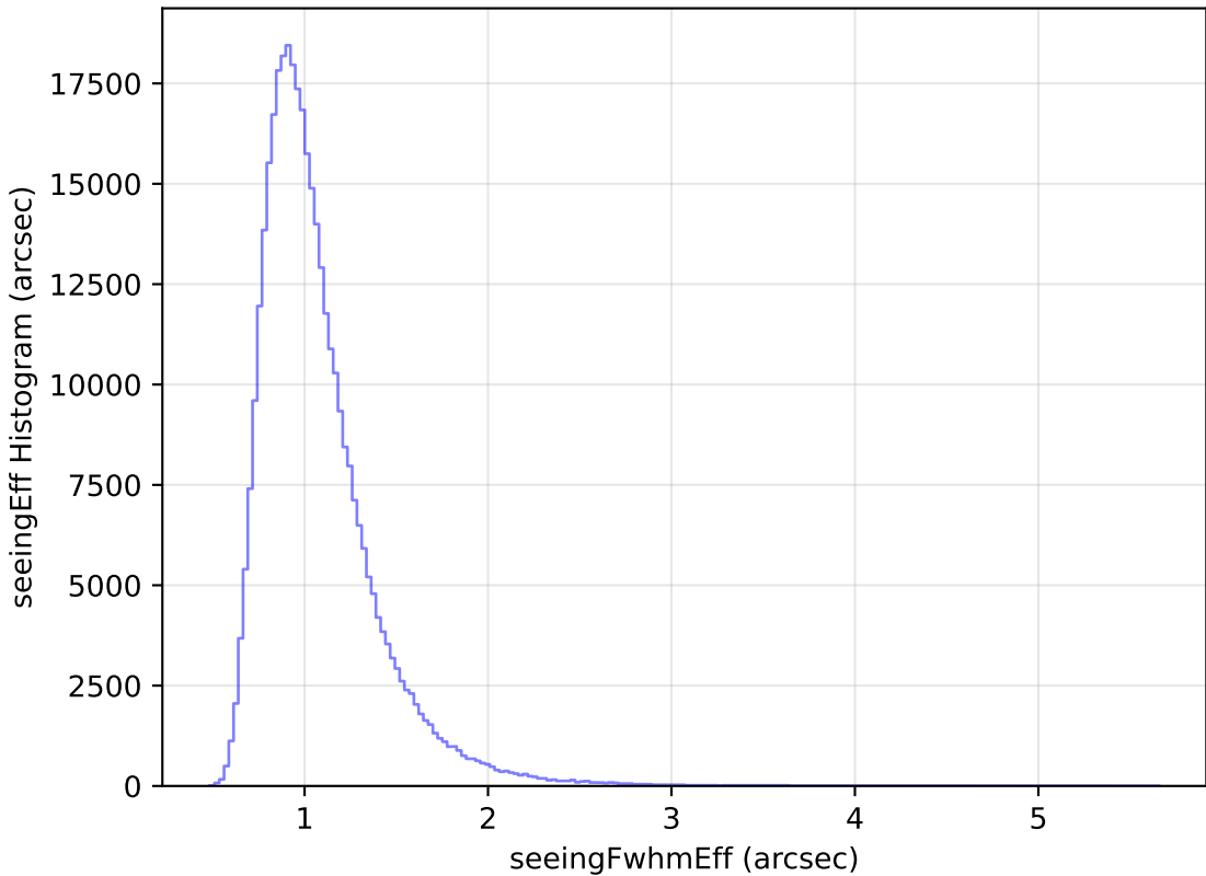
roll_pause_mjdp0_v3.4_10yrs WFD y band: seeingEff Histogram
