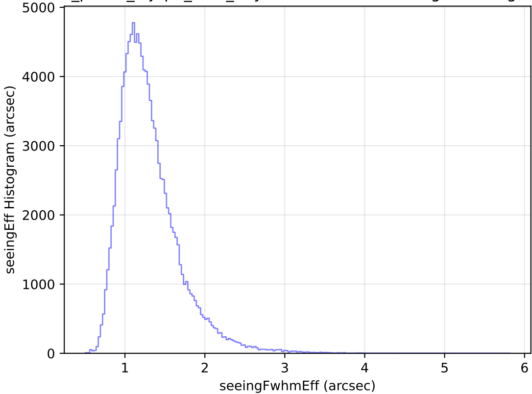
roll_pause_mjdp0_v3.4_10yrs WFD u band: seeingEff Histogram
