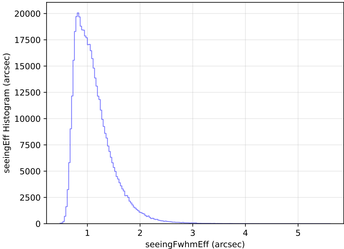
roll_pause_mjdp0_v3.4_10yrs WFD r band: seeingEff Histogram
