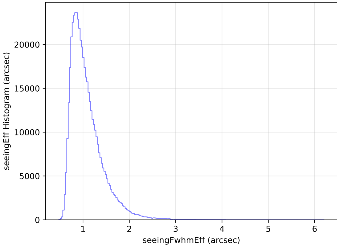
roll_pause_mjdp0_v3.4_10yrs WFD i band: seeingEff Histogram
