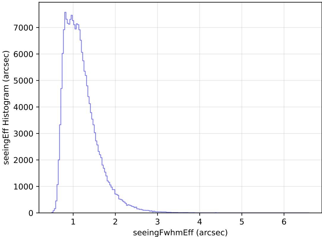
roll_pause_mjdp0_v3.4_10yrs WFD g band: seeingEff Histogram
