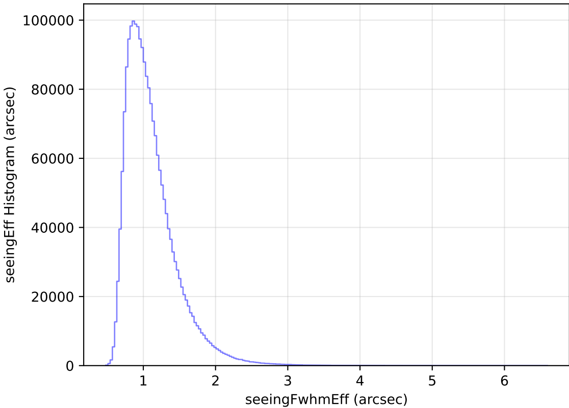
roll_pause_mjdp0_v3.4_10yrs WFD all bands: seeingEff Histogram
