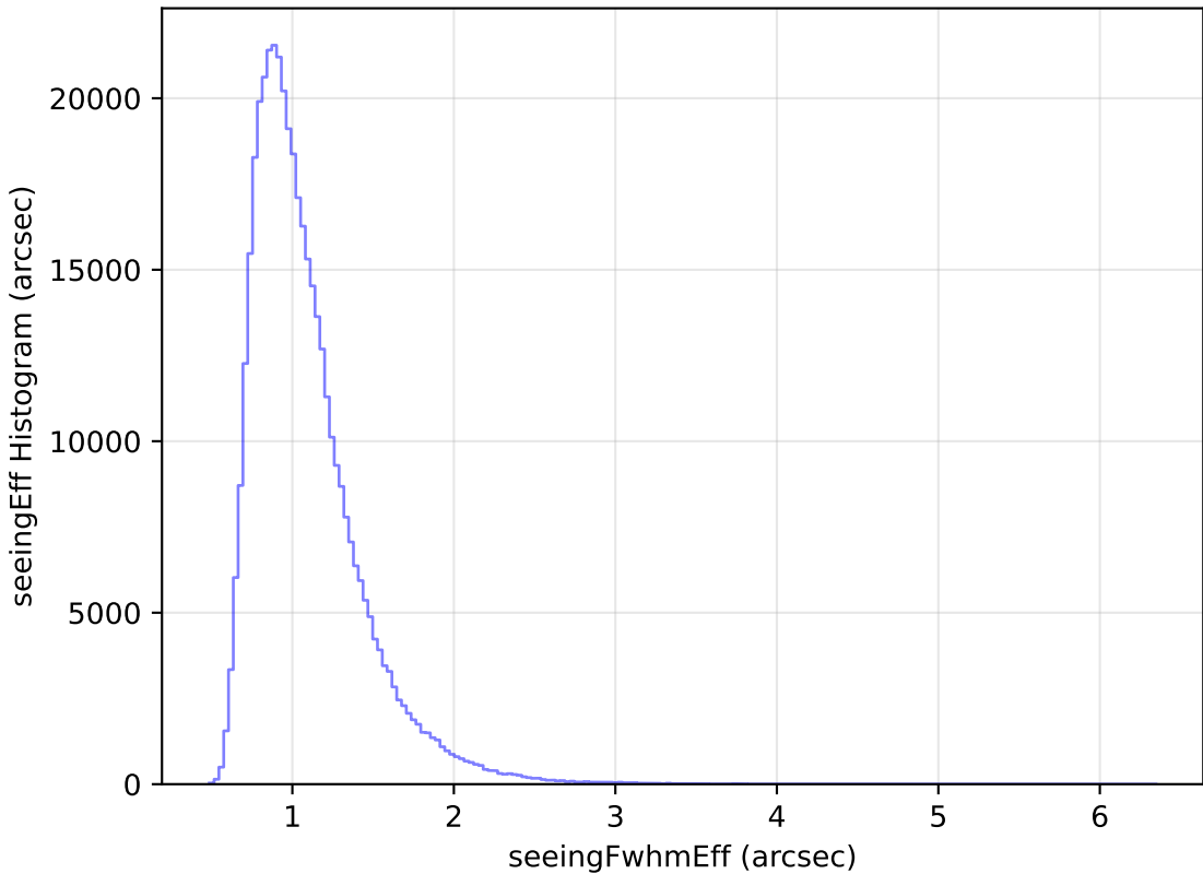
roll_pause_mjdp0_v3.4_10yrs All sky z band: seeingEff Histogram
