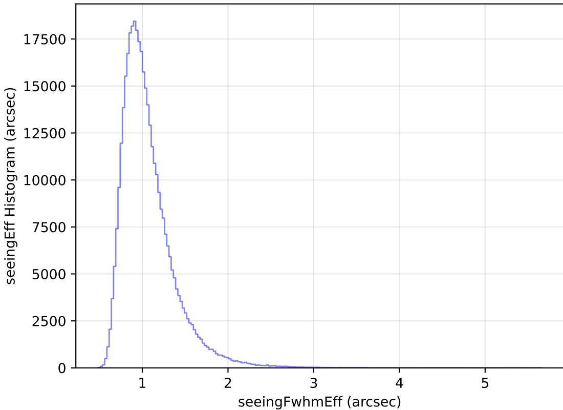
roll_pause_mjdp0_v3.4_10yrs All sky y band: seeingEff Histogram
