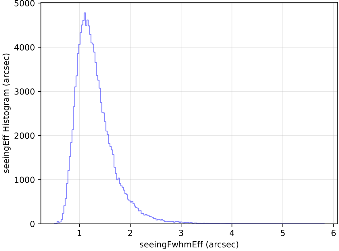
roll_pause_mjdp0_v3.4_10yrs All sky u band: seeingEff Histogram
