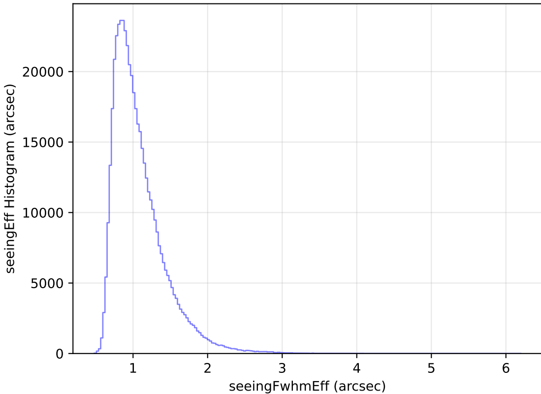
roll_pause_mjdp0_v3.4_10yrs All sky i band: seeingEff Histogram
