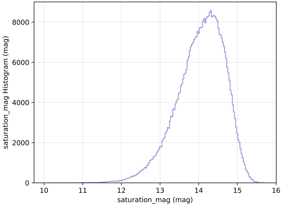
roll_pause_mjdp0_v3.4_10yrs WFD z band: saturation_mag Histogram
