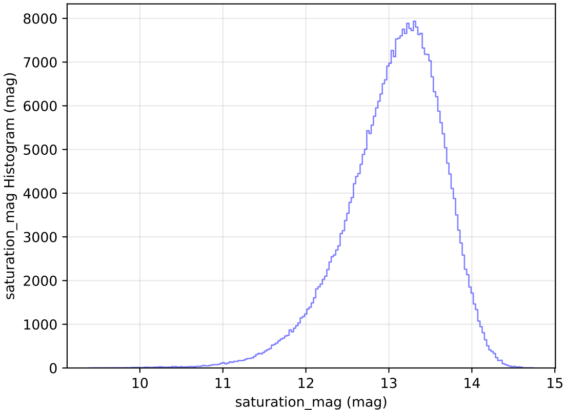
roll_pause_mjdp0_v3.4_10yrs WFD y band: saturation_mag Histogram
