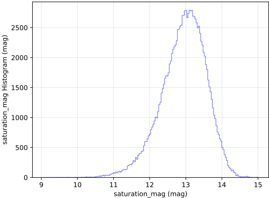
roll_pause_mjdp0_v3.4_10yrs WFD u band: saturation_mag Histogram
