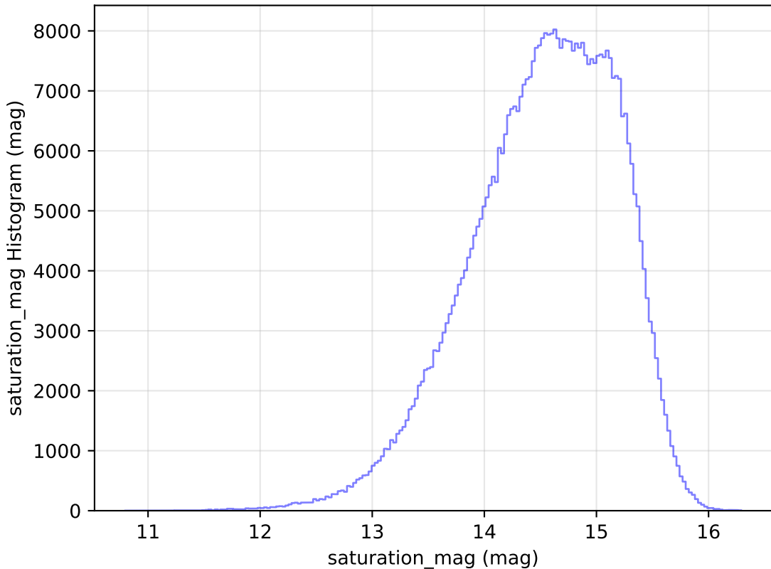
roll_pause_mjdp0_v3.4_10yrs WFD r band: saturation_mag Histogram
