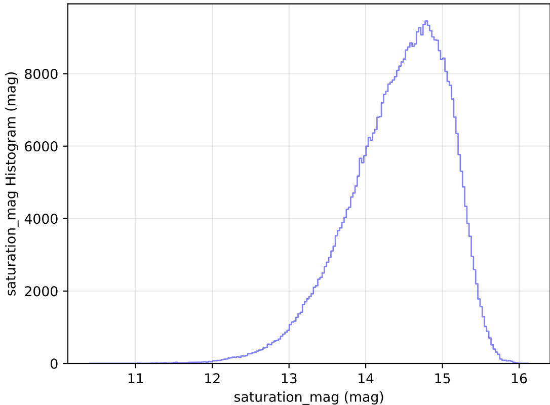
roll_pause_mjdp0_v3.4_10yrs WFD i band: saturation_mag Histogram
