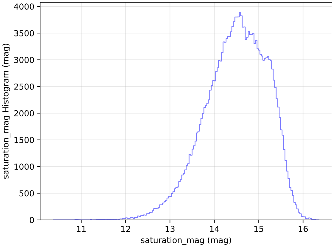
roll_pause_mjdp0_v3.4_10yrs WFD g band: saturation_mag Histogram
