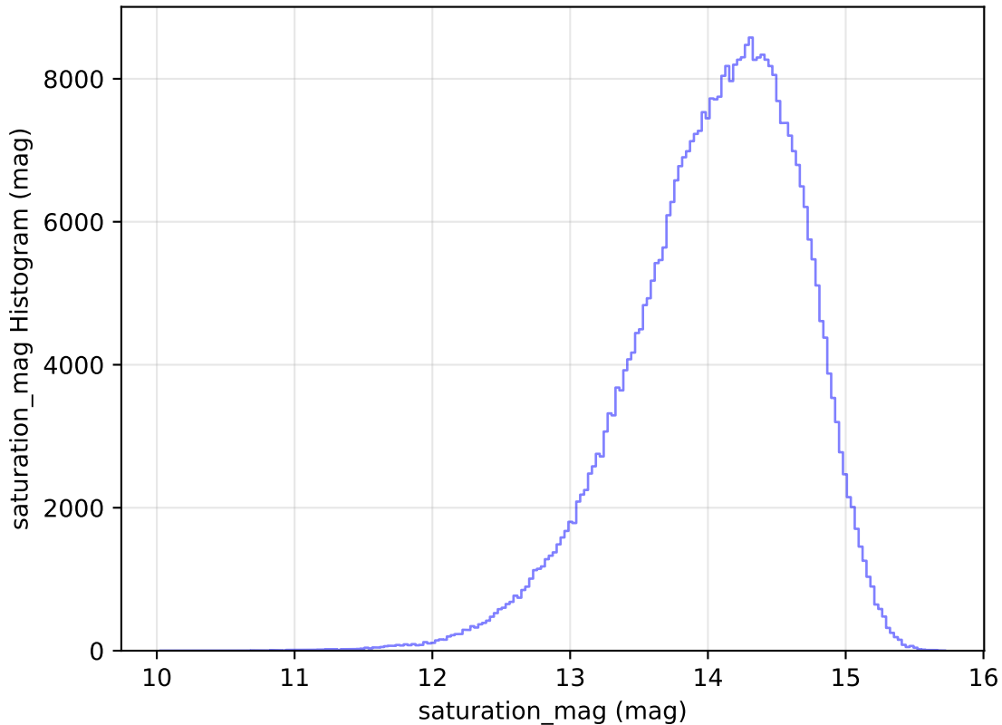
roll_pause_mjdp0_v3.4_10yrs All sky z band: saturation_mag Histogram
