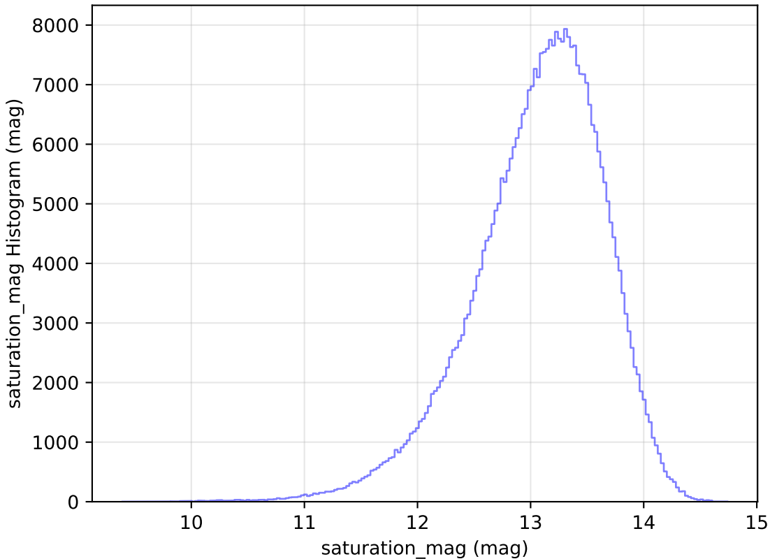
roll_pause_mjdp0_v3.4_10yrs All sky y band: saturation_mag Histogram
