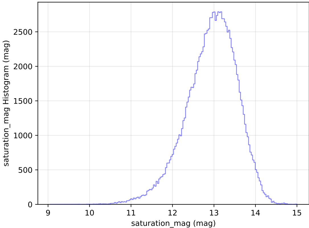
roll_pause_mjdp0_v3.4_10yrs All sky u band: saturation_mag Histogram
