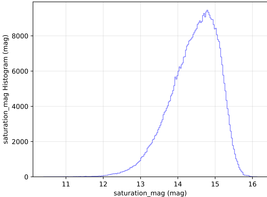
roll_pause_mjdp0_v3.4_10yrs All sky i band: saturation_mag Histogram
