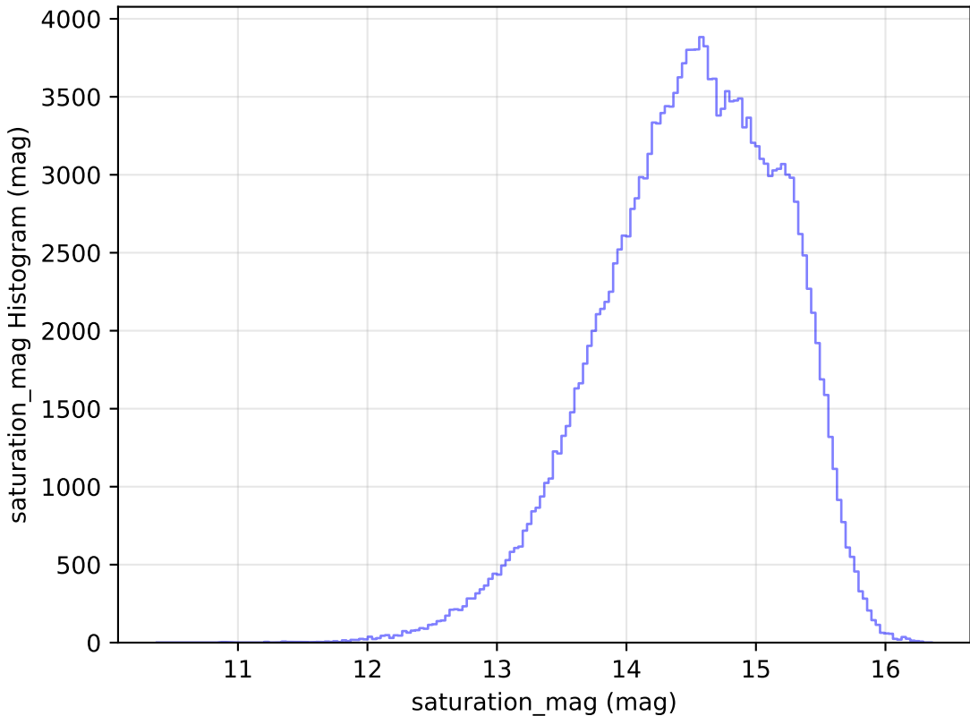
roll_pause_mjdp0_v3.4_10yrs All sky g band: saturation_mag Histogram
