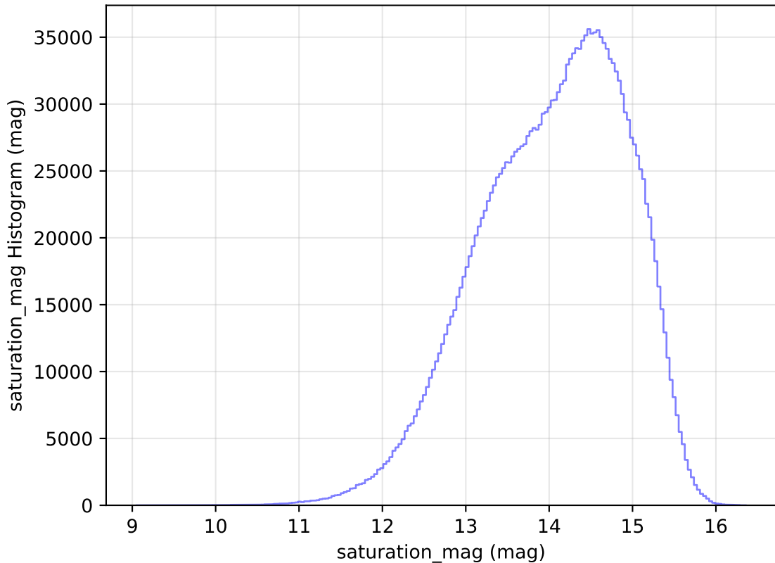
roll_pause_mjdp0_v3.4_10yrs All sky all bands: saturation_mag Histogram
