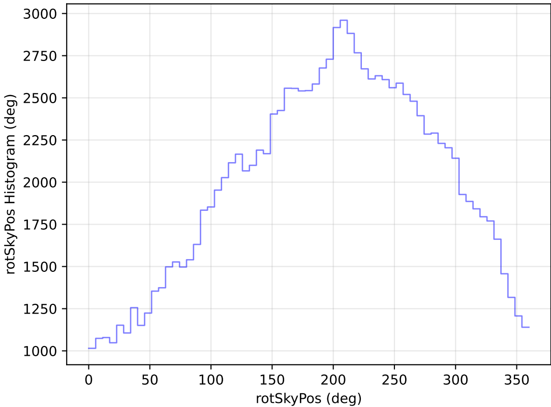
roll_pause_mjdp0_v3.4_10yrs WFD u band: rotSkyPos Histogram
