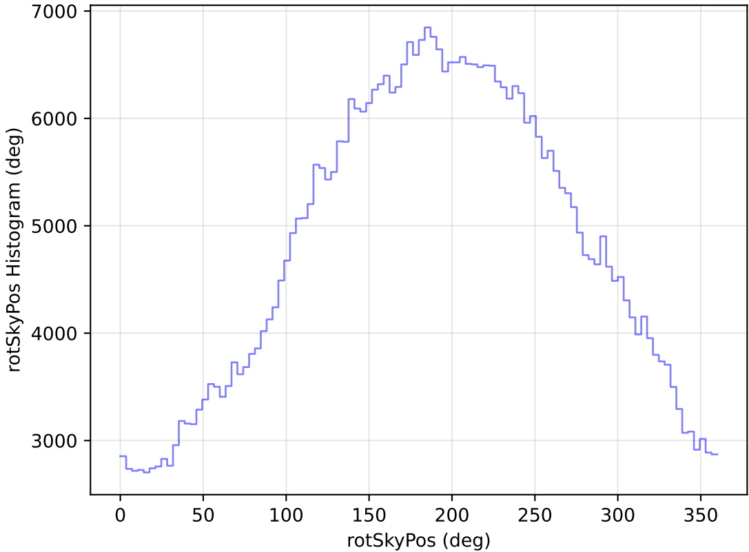
roll_pause_mjdp0_v3.4_10yrs WFD r band: rotSkyPos Histogram
