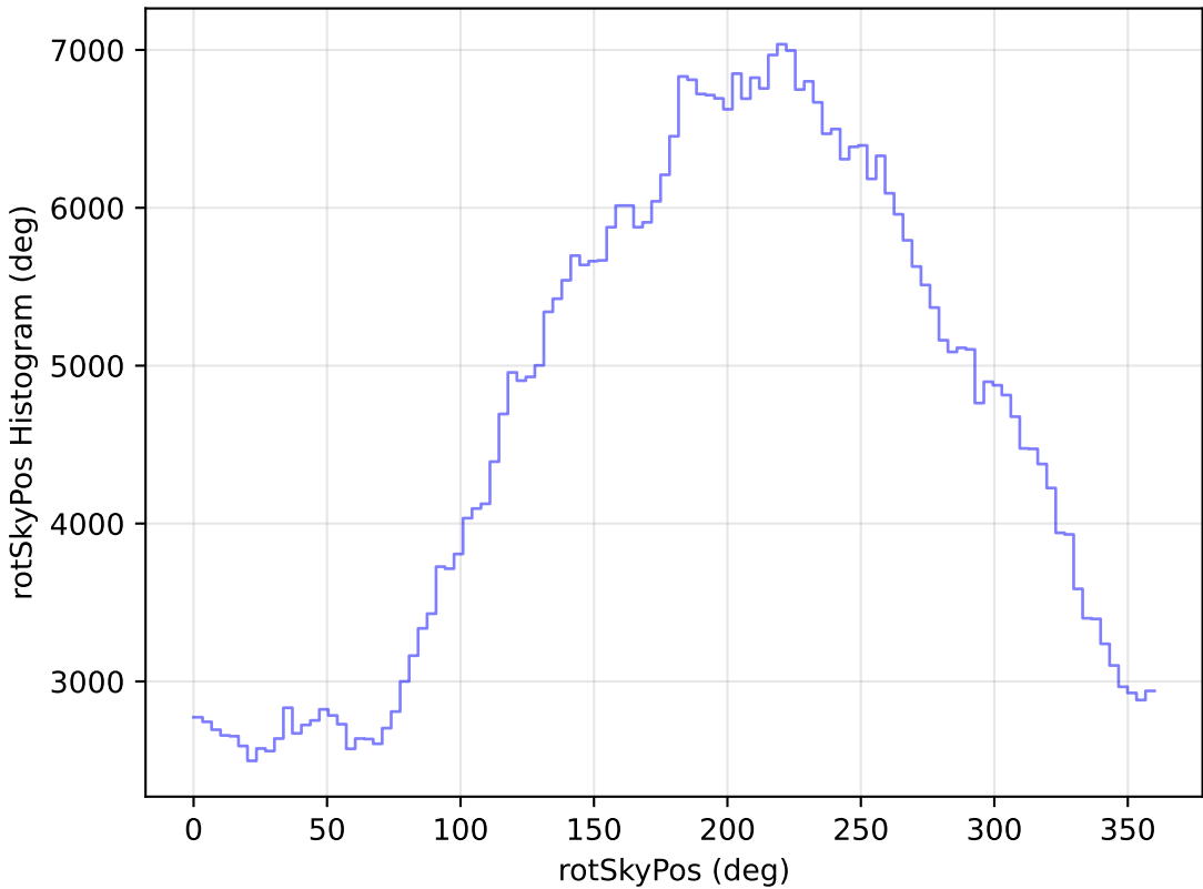
roll_pause_mjdp0_v3.4_10yrs WFD i band: rotSkyPos Histogram
