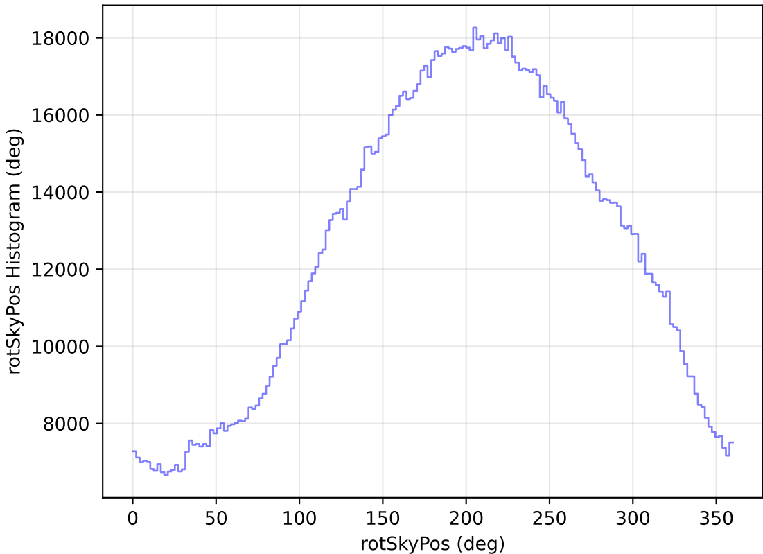
roll_pause_mjdp0_v3.4_10yrs WFD all bands: rotSkyPos Histogram
