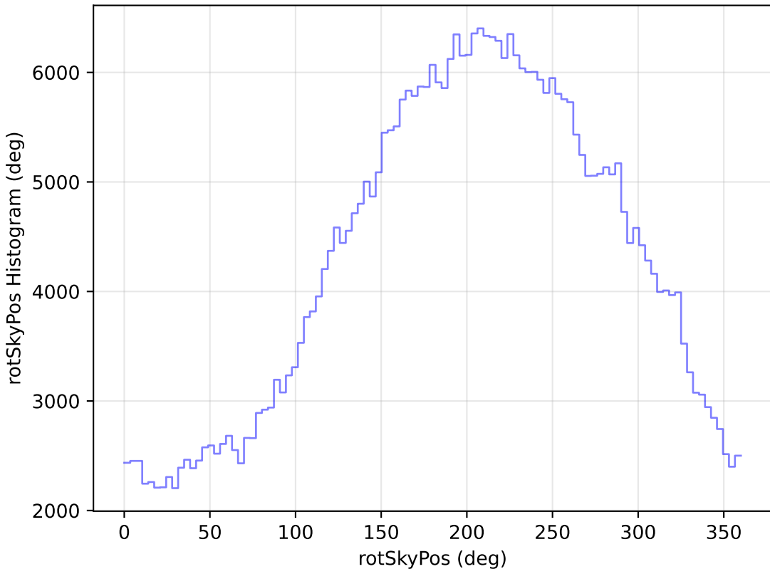
roll_pause_mjdp0_v3.4_10yrs All sky z band: rotSkyPos Histogram
