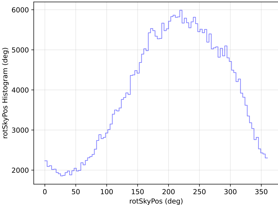
roll_pause_mjdp0_v3.4_10yrs All sky y band: rotSkyPos Histogram
