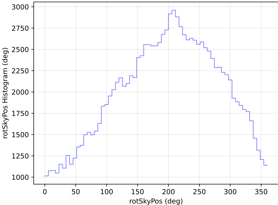
roll_pause_mjdp0_v3.4_10yrs All sky u band: rotSkyPos Histogram
