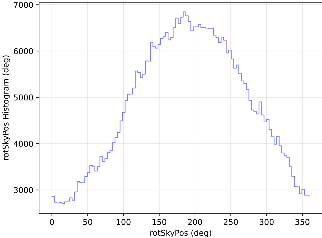
roll_pause_mjdp0_v3.4_10yrs All sky r band: rotSkyPos Histogram
