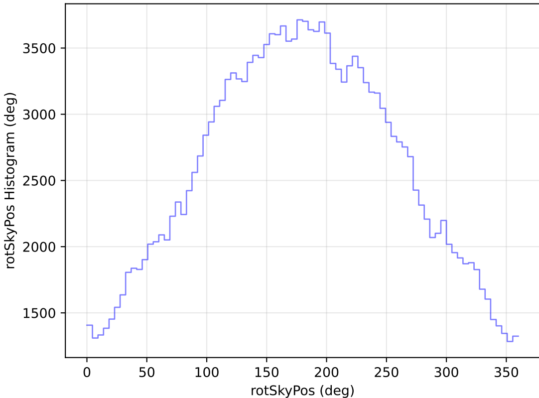
roll_pause_mjdp0_v3.4_10yrs All sky g band: rotSkyPos Histogram
