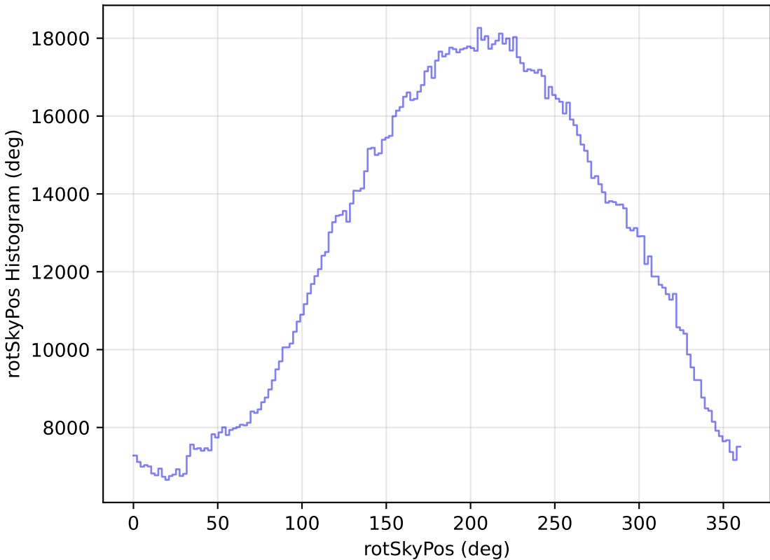
roll_pause_mjdp0_v3.4_10yrs All sky all bands: rotSkyPos Histogram
