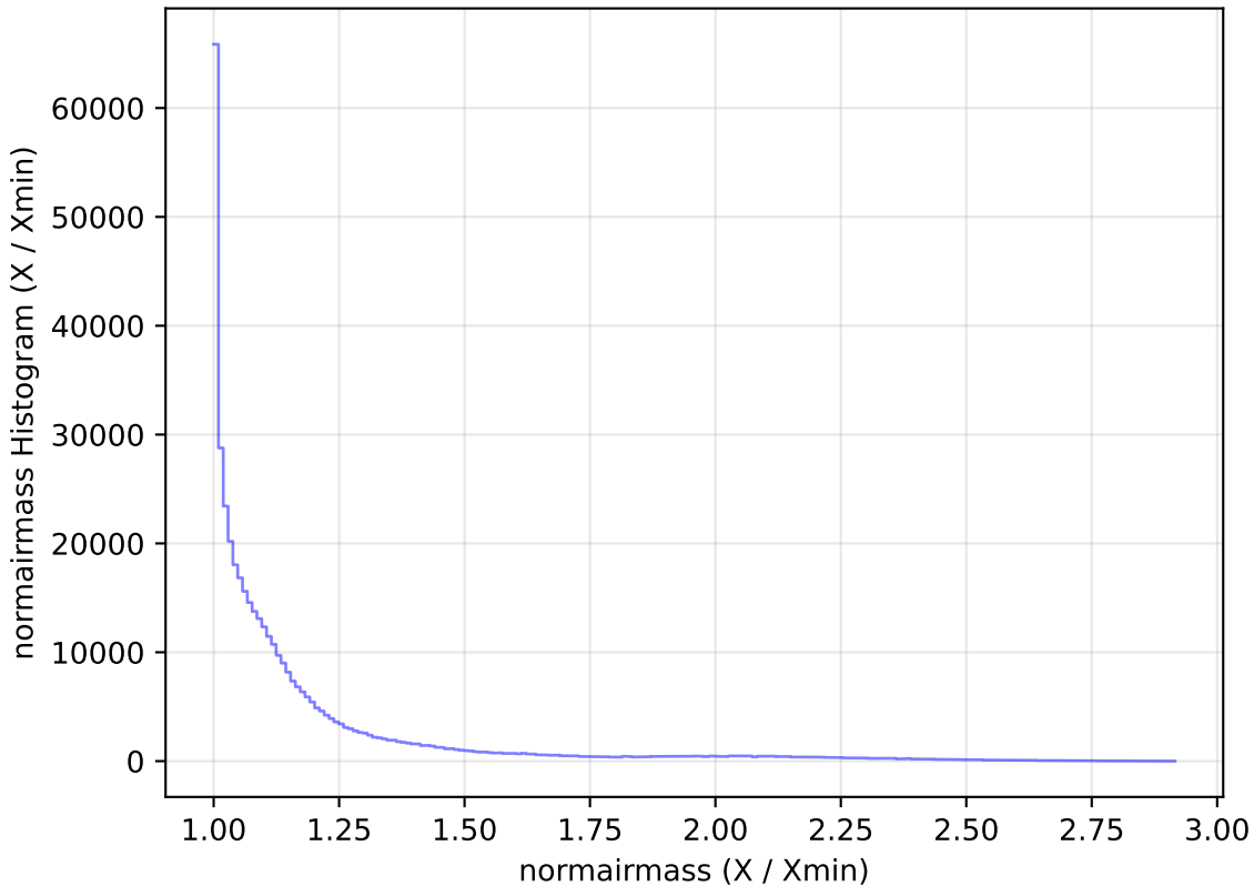
roll_pause_mjdp0_v3.4_10yrs WFD z band: normairmass Histogram
