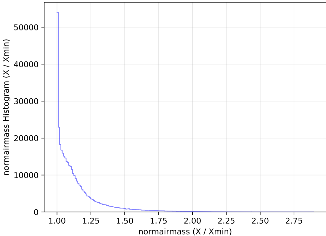
roll_pause_mjdp0_v3.4_10yrs WFD y band: normairmass Histogram
