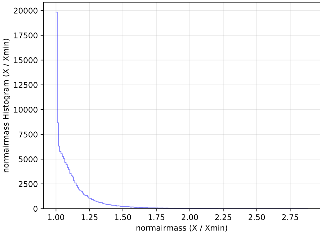
roll_pause_mjdp0_v3.4_10yrs WFD u band: normairmass Histogram
