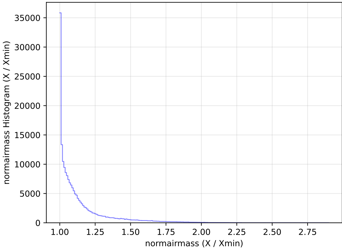
roll_pause_mjdp0_v3.4_10yrs WFD g band: normairmass Histogram
