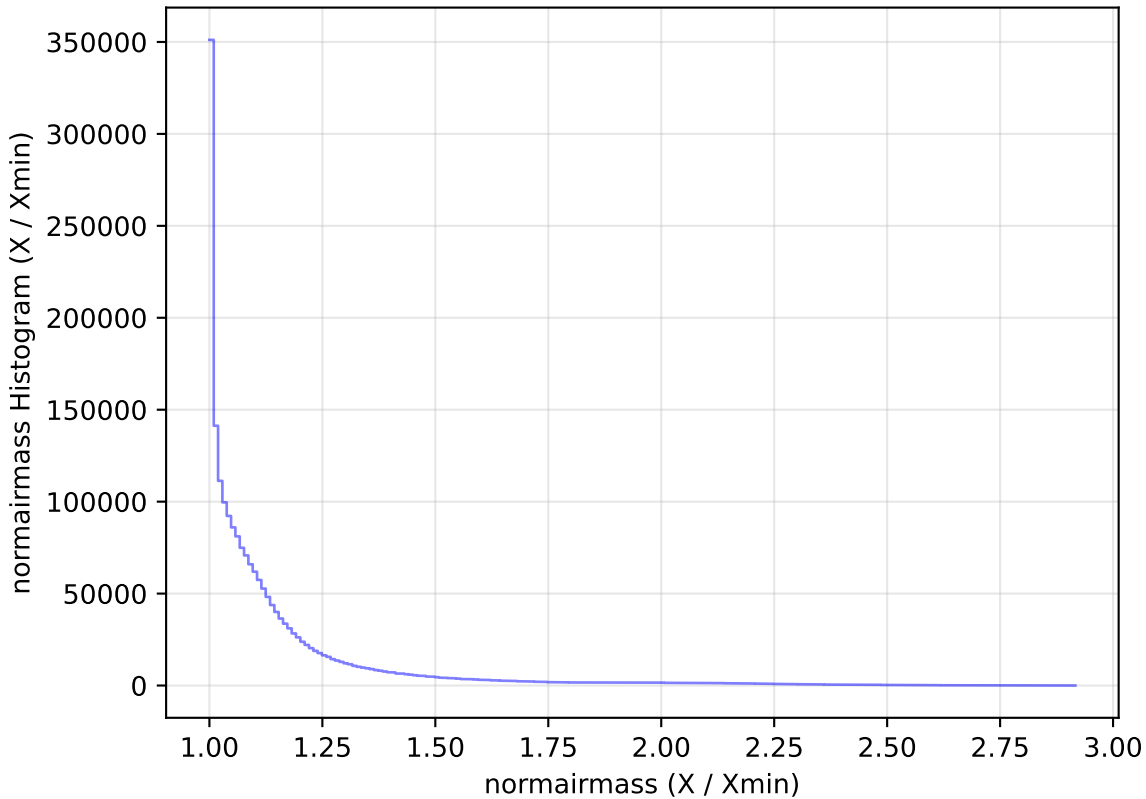
roll_pause_mjdp0_v3.4_10yrs WFD all bands: normairmass Histogram
