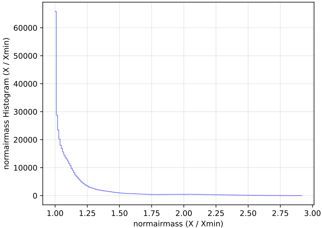
roll_pause_mjdp0_v3.4_10yrs All sky z band: normairmass Histogram
