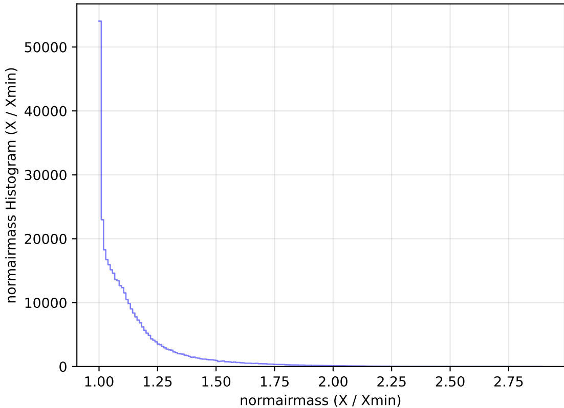
roll_pause_mjdp0_v3.4_10yrs All sky y band: normairmass Histogram
