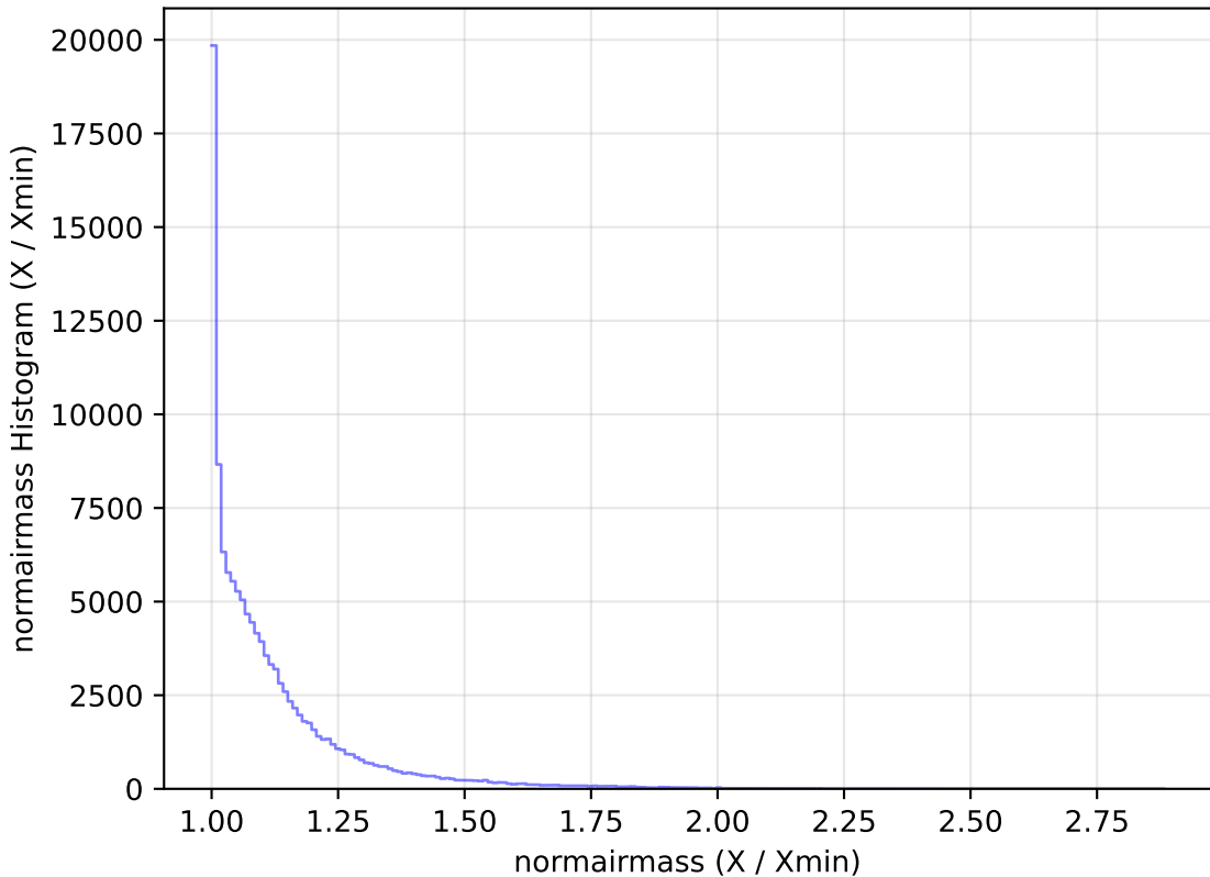
roll_pause_mjdp0_v3.4_10yrs All sky u band: normairmass Histogram
