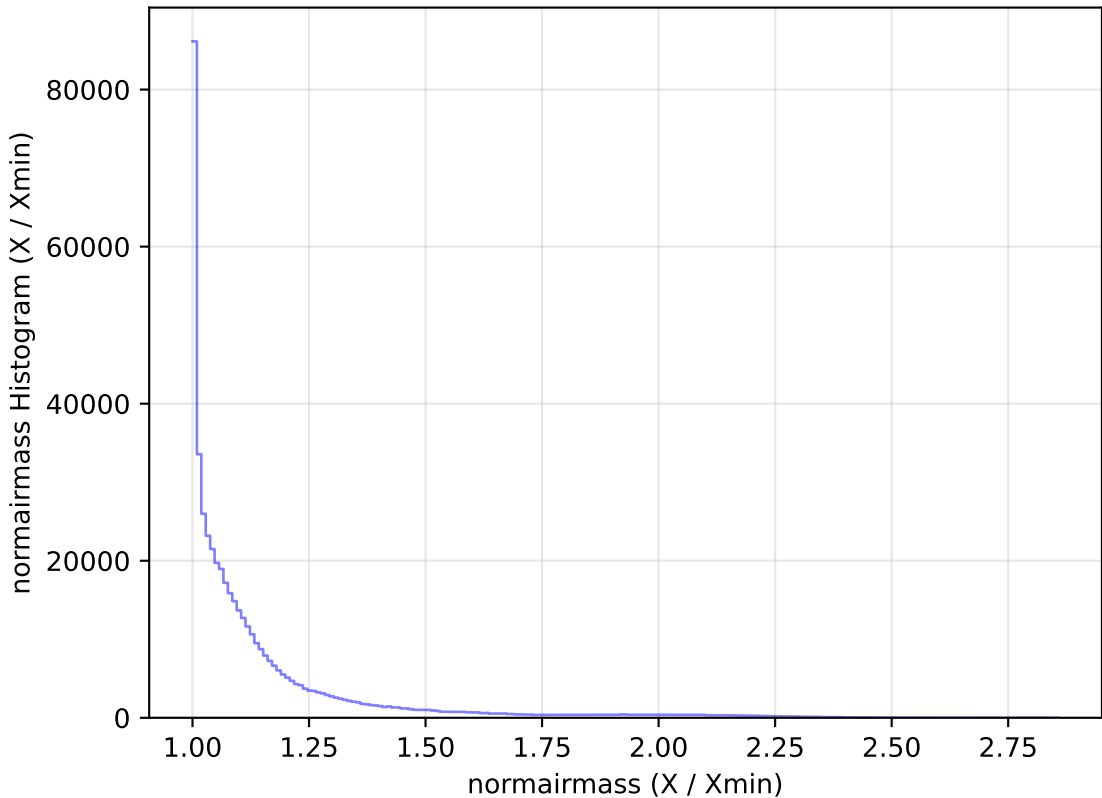
roll_pause_mjdp0_v3.4_10yrs All sky r band: normairmass Histogram
